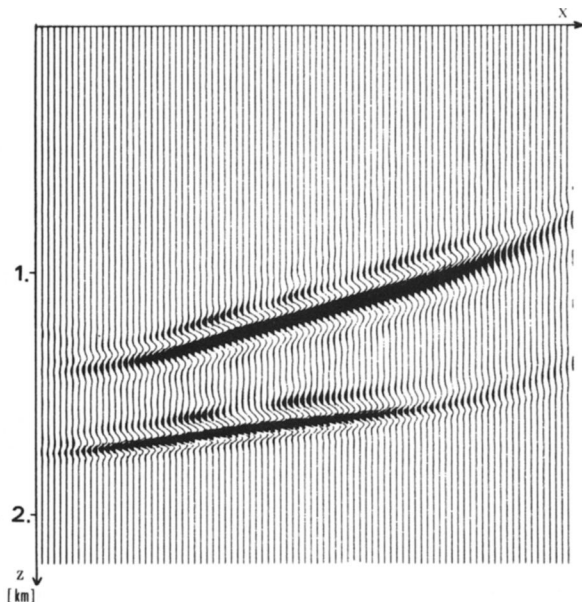
FIG. 9. Wave-equation migration, results for the three-layered model.
